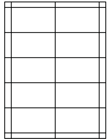
HS-2000-AB & HS-2000-M 10-up layout from 8-1/2" x 11" 1/2" trim top and bottom, 3/4" trim sides
