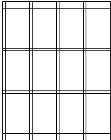
HS-3000-GC 12-up layout from 9" x 12" Gutter Cut: 1/4" and 1/8" between cards, 1/8" sides, 1/2" top and bottom
